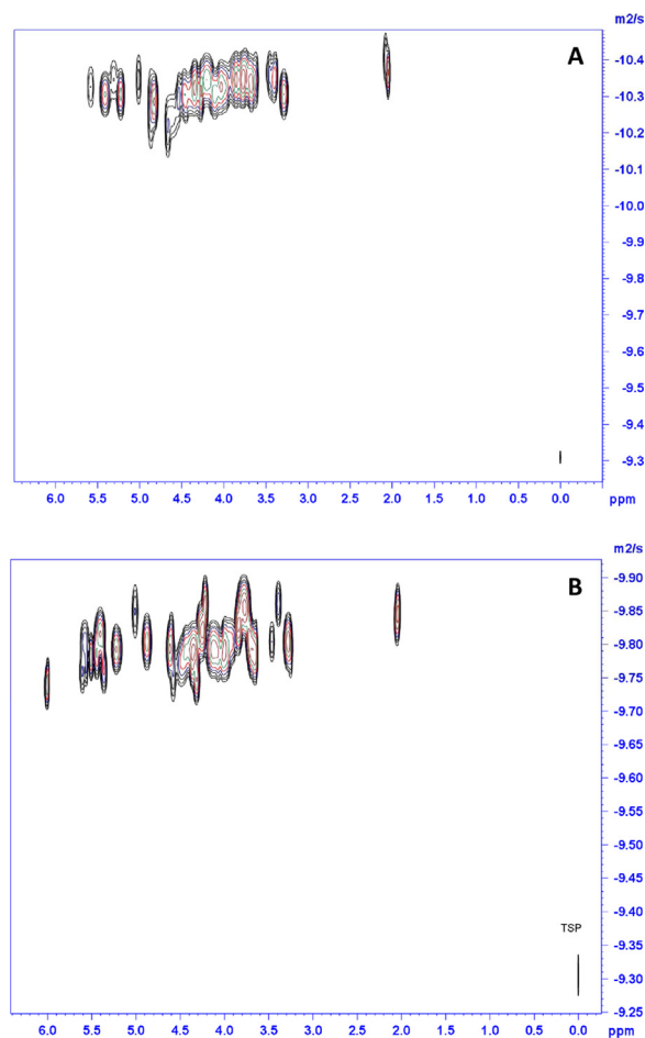
Fig. 1. Representative DOSY spectra of porcine heparin (A) and porcine LMWH (B).
