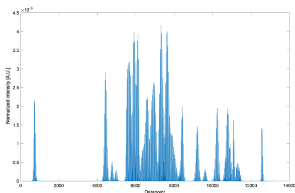
Fig. 2. Unfolded spectral data of porcine LMWH sample (
